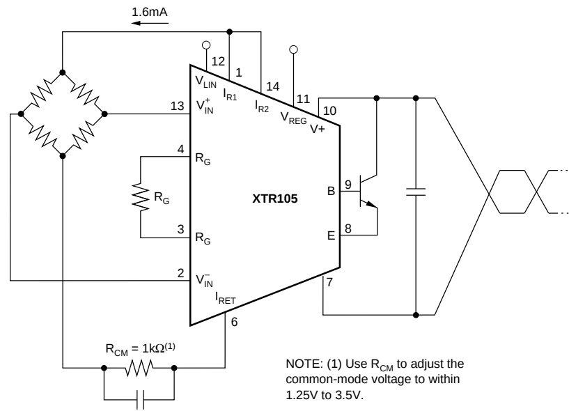
FIGURE 9. Bridge Input, Current Excitation.
