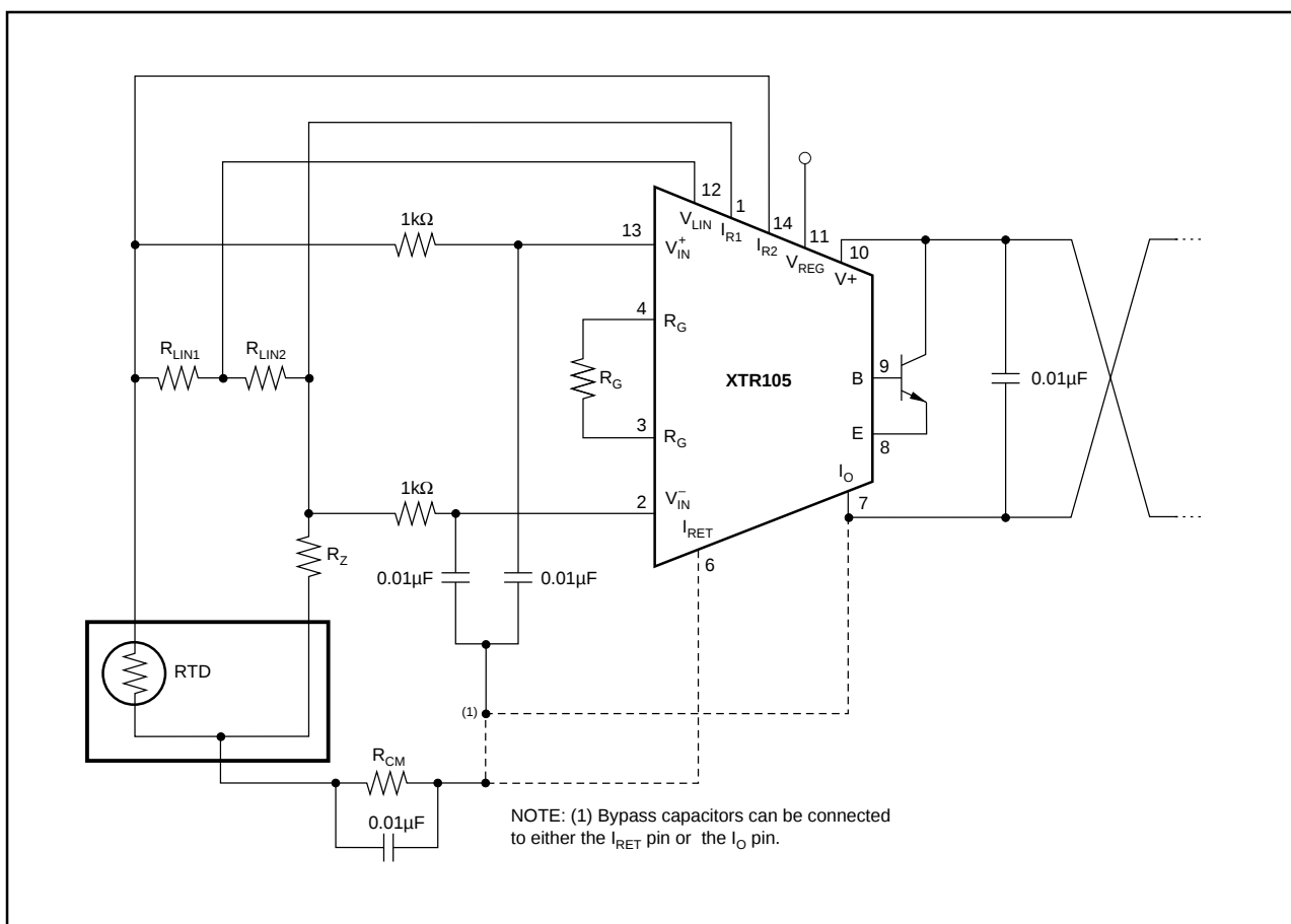
FIGURE 5. Input Bypassing Technique with Linearization.
