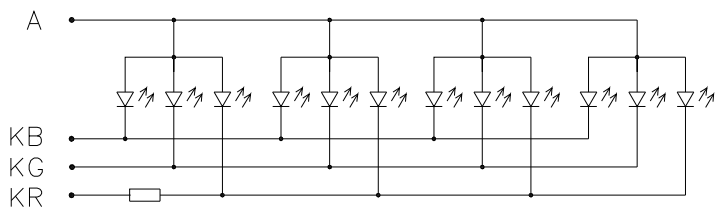
CIRCUIT DIAGRAM
