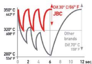
Process for 3 solder joints
