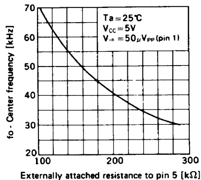
Center frequency characteristics vs. Externally attached resistance
