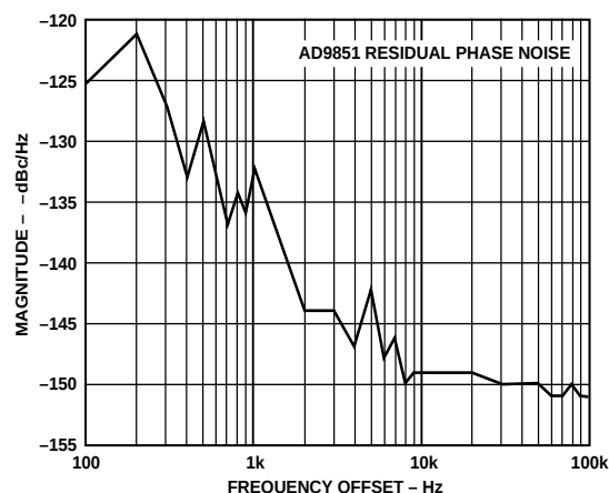
Figure 36. Output Residual Phase Noise (5.2 MHz A_{OUT} ), 6 \times \text{REFCLK} Multiplier Disabled, System Clock = 180 MHz, Reference Clock = 180 MHz
