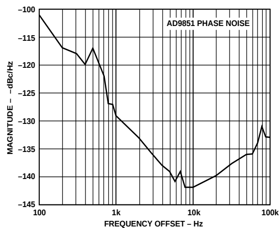
Figure 35. Output Phase Noise (5.2 MHz A_{OUT} ), 6 \times \text{REFCLK} Multiplier Enabled, System Clock = 180 MHz, Reference Clock = 30 MHz
