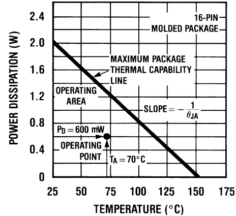
FIGURE 5. Package Power Capability vs Temperature
