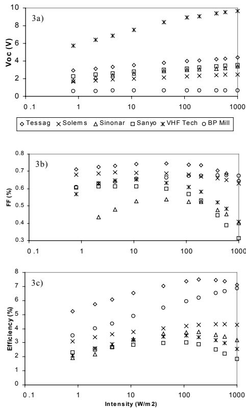
Figure 3 a), b) & c): Comparison of amorphous silicon solar cells over four orders of magnitude of intensity below AM1.5 ( 1000\text{W/m}^2 )
