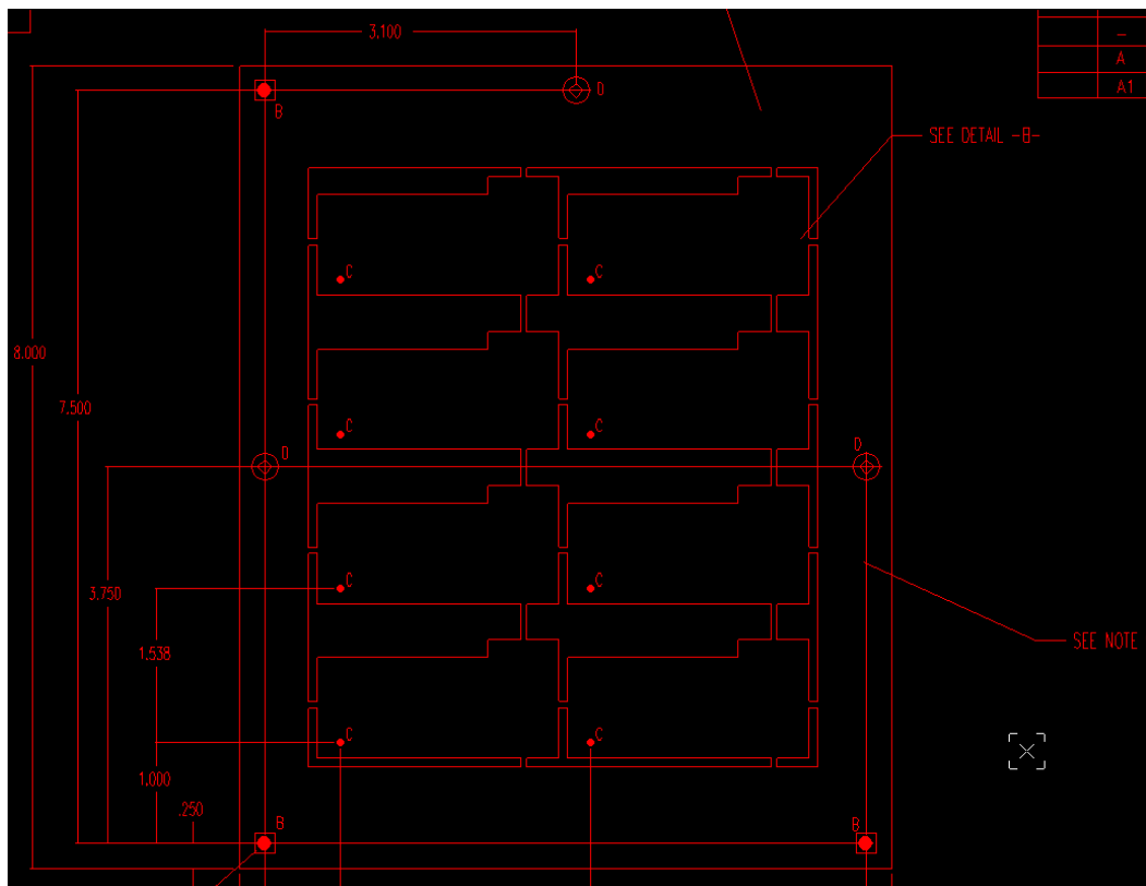
Fig 8 Tab-routing panel
