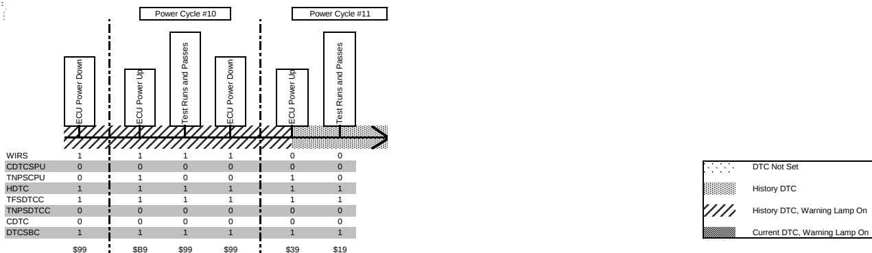
Figure E9: Powertrain Type A DTC (3 of 3)
