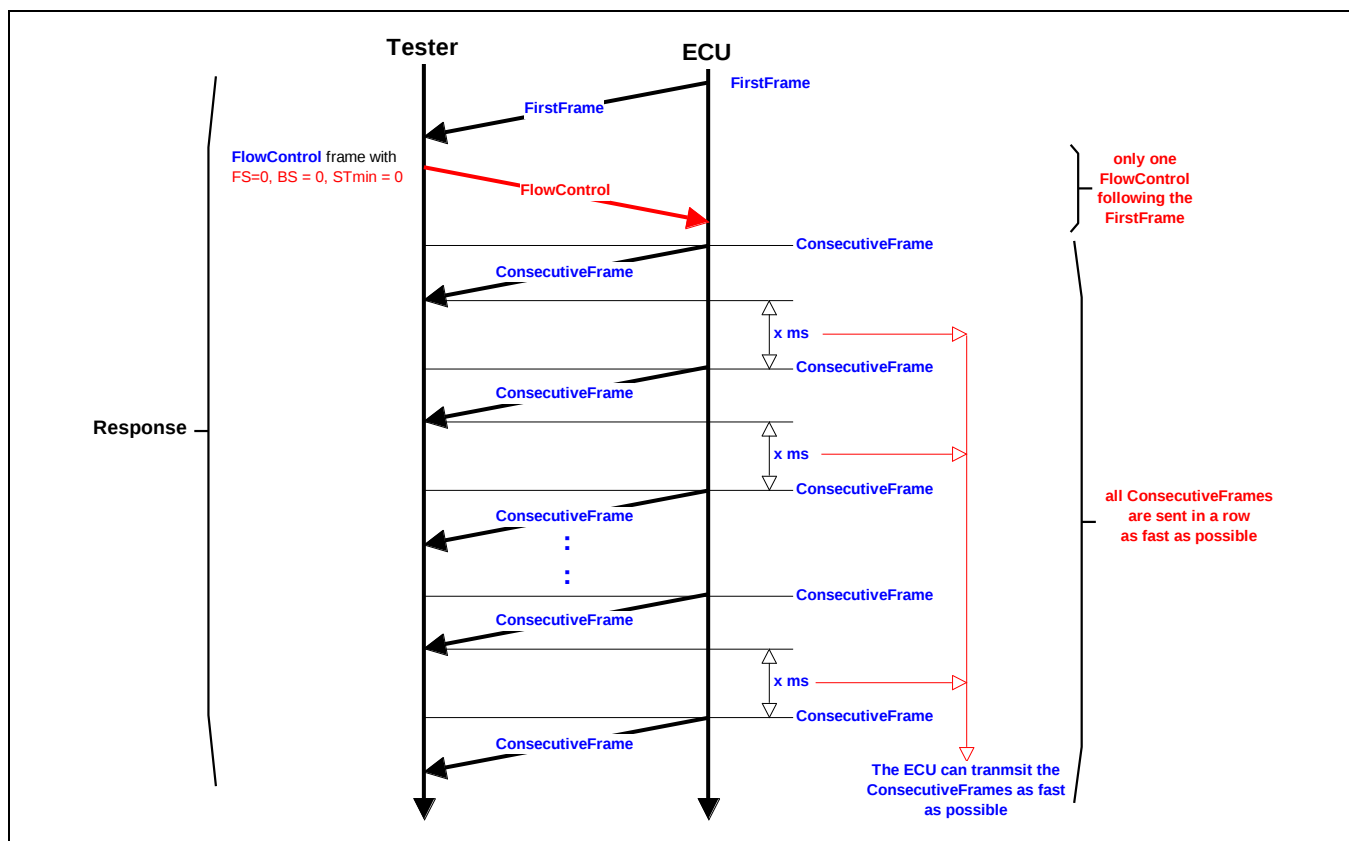
Figure 31: Tester Requirements for Multi-Frame Response Messages - Example Message Flow
