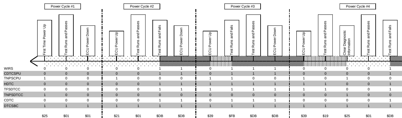
Figure E3: Limited Duration Latching DTC (1 of 2)
