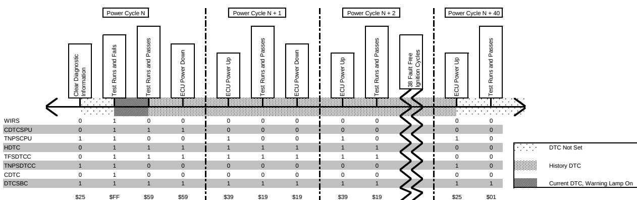
Figure E15: Automatic Clearing of DTCs
