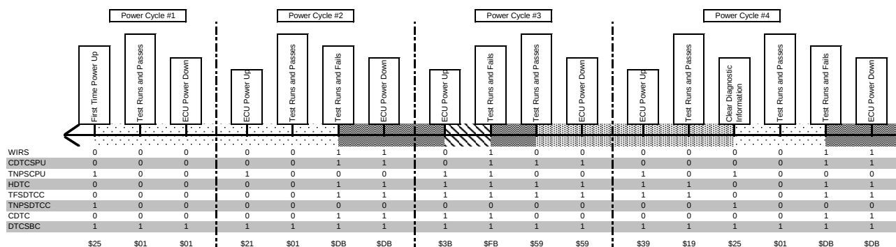
Figure E13: Powertrain Type C DTC (1 of 2)
