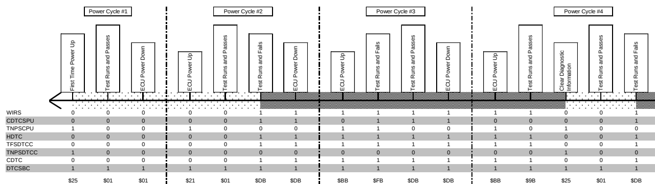
Figure E5: Permanently Latched DTC (1 of 2)
