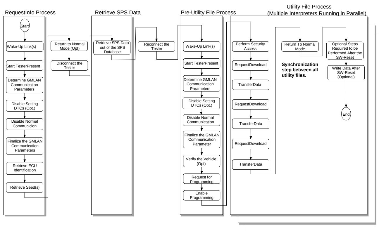
Figure 40: Programming Procedure – Summary
