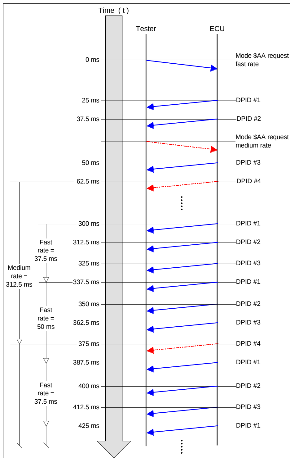
Figure 35: Example #2 - Mixture of DPID Schedule Rates
