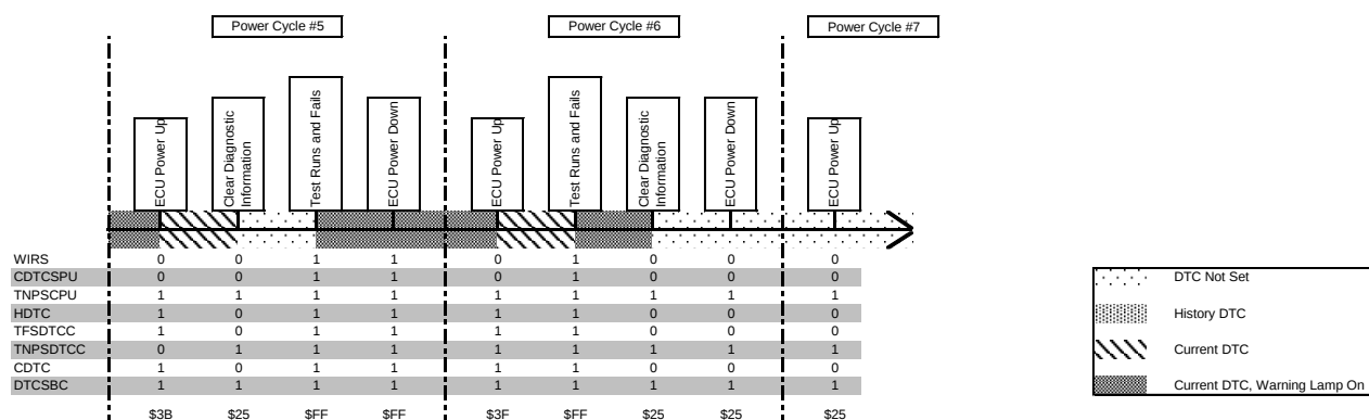
Figure E14: Powertrain Type C DTC (2 of 2)
