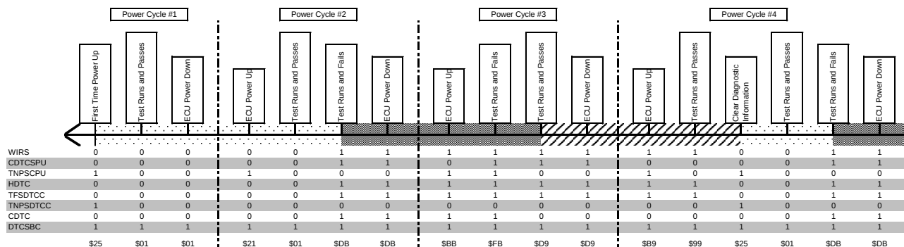
Figure E7: Powertrain Type A DTC (1 of 3)
